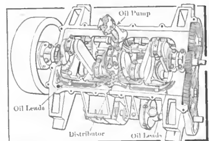
Fig. 4—Looking into the crankcase of the Stoddard-Dayton from below, showing oil leads
